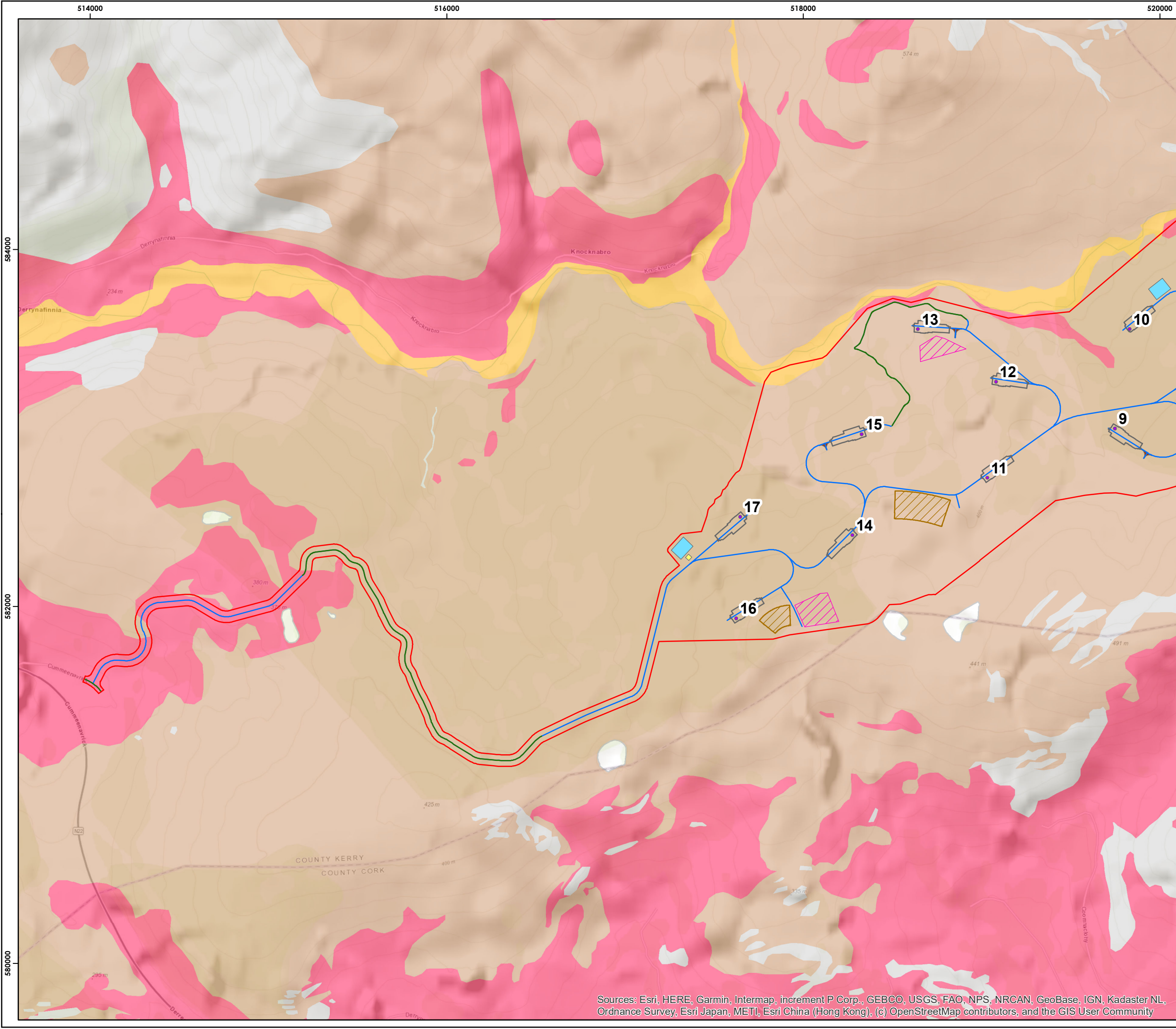
Figure 10-2a Quaternary Sediments
